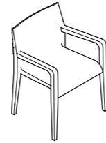
LALEGGERA ARMREST cm 49x56 - h cm 79 - h seat cm 45
